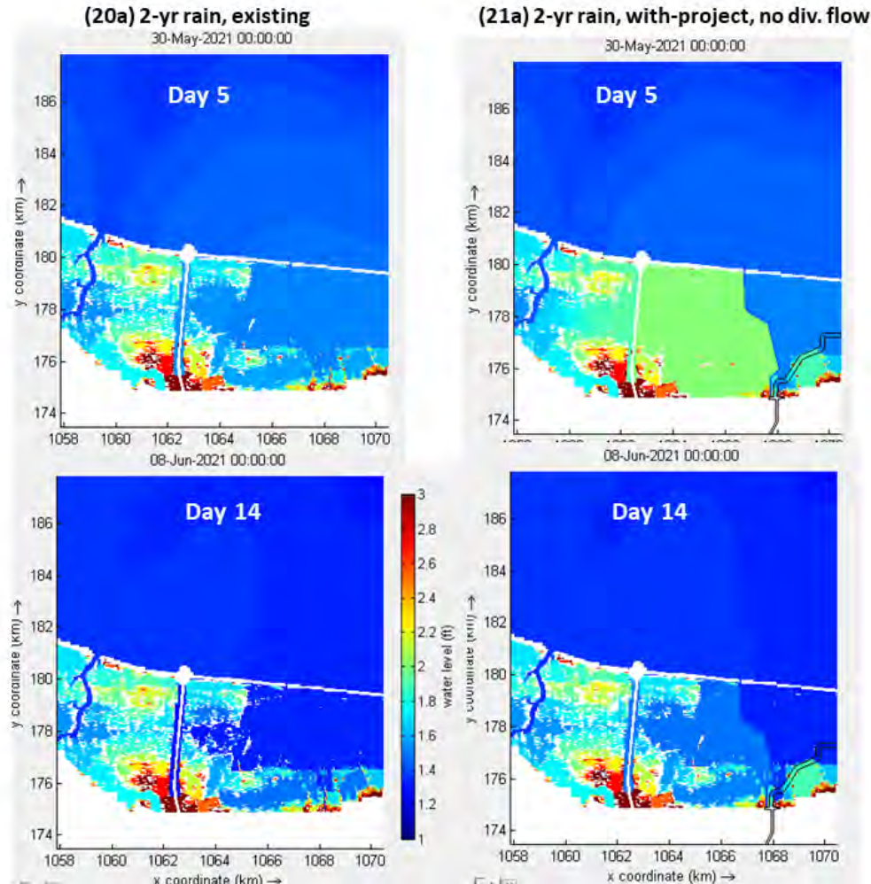
Figure G2. Comparison of existing and with-project, no diversion flow conditions (2-year rainfall).
