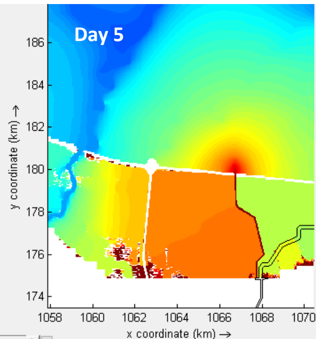
(22b) 25-yr rain, with-project, div. 2000 cfs
