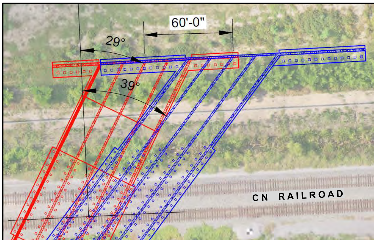
Figure 6.6 – Culvert Skew Angles v/v 60-ft Shift of Alignment at CN RR
