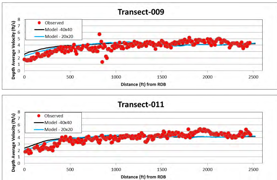
FigureA-5. Comparison between CFD model and field data at transects #009 and #0011. Red dots show the field data and model results are given for two different meshes – 40x40 feet in size and 20x20 feet in size. The results with either mesh are similar.
