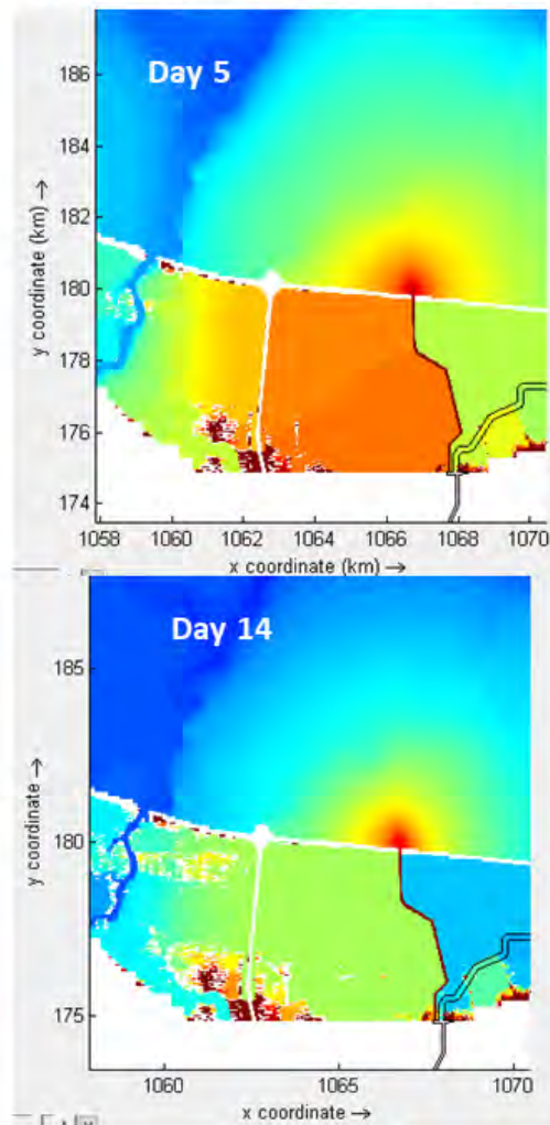
25-yr rain, with-project, div flow 2000 cfs
