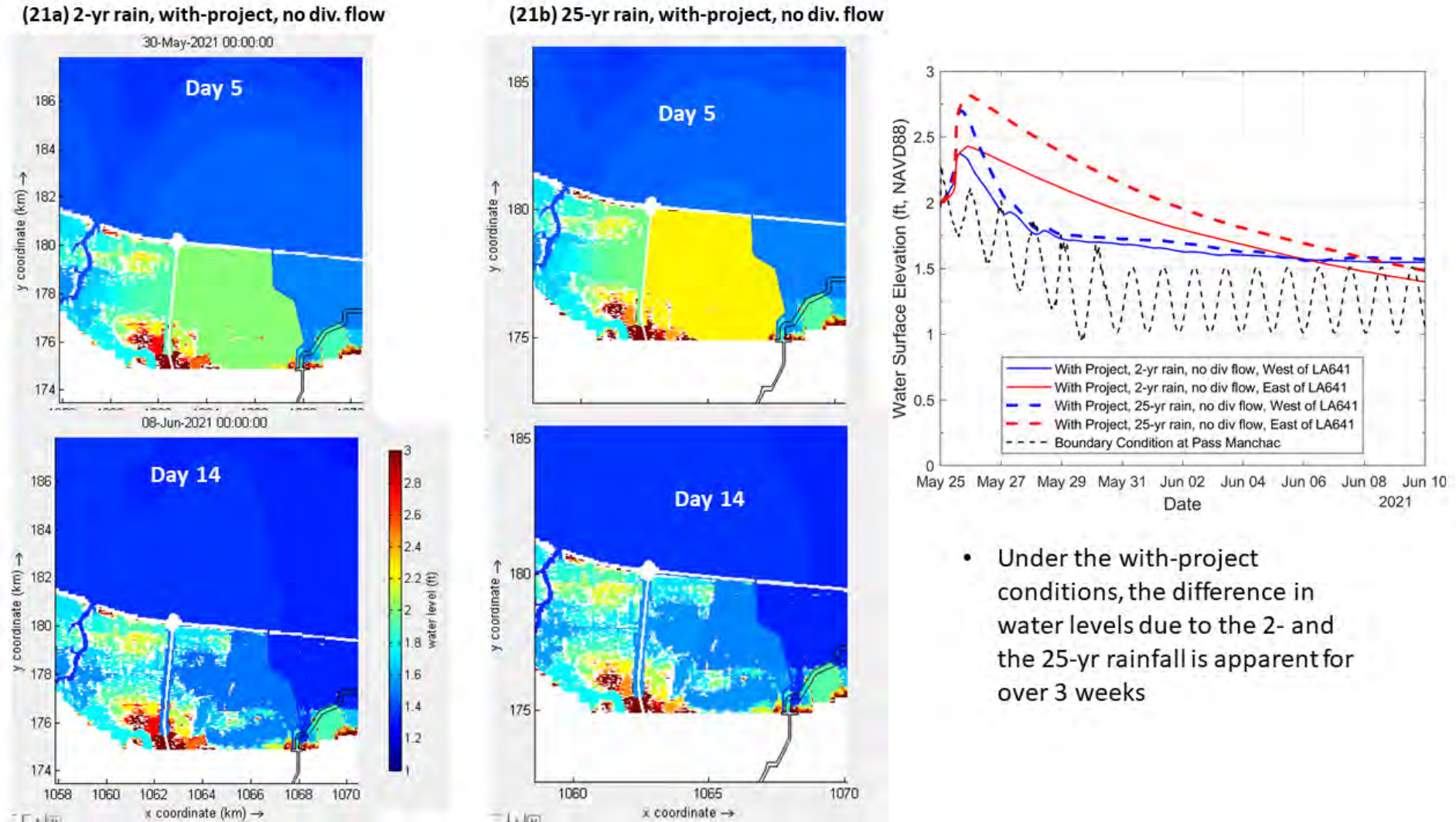
Figure G9. Comparison of with-project, no diversion flow conditions under 2-year and 25-year rainfall.
