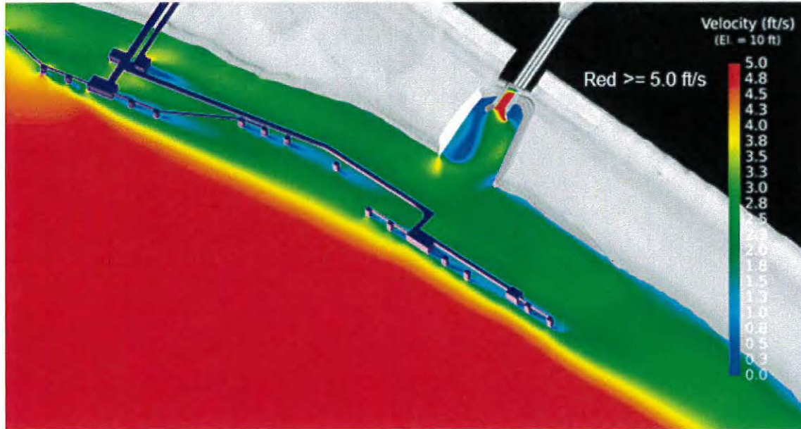
Figure 5 – Velocity contours with previous docking facility and operating diversion. Slice plane cut horizontally at an elevation equal to 10 ft.
