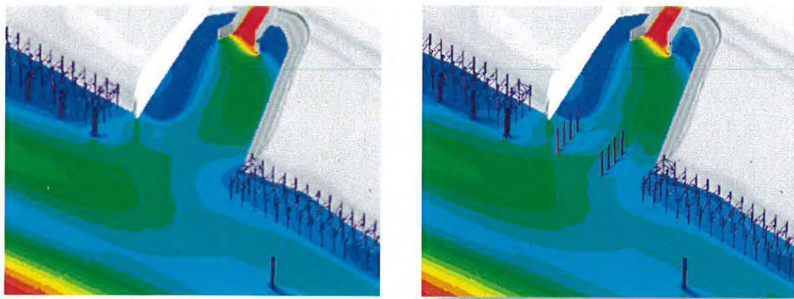
Figure 29 – Comparison of velocity contours at the entrance of the diversion channel between Alternative 1 (left) and Alternative 2 (right) docking facilities. Slice plane cut horizontally at an elevation equal to 10 ft.
