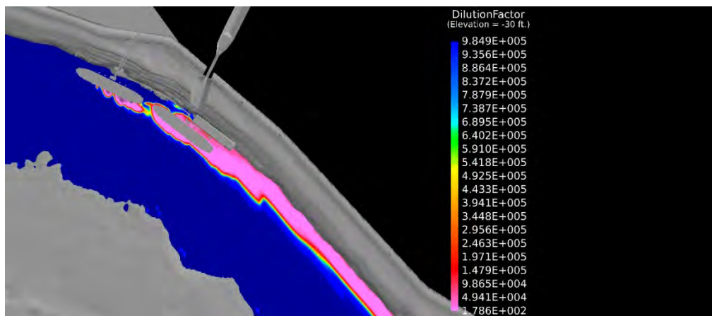
Figure A-21. Run #10 model results. Dilution factors at elevations 22 feet (top), 0 feet (middle), and -30 feet (bottom) 1 hour after Bitumen spill.
