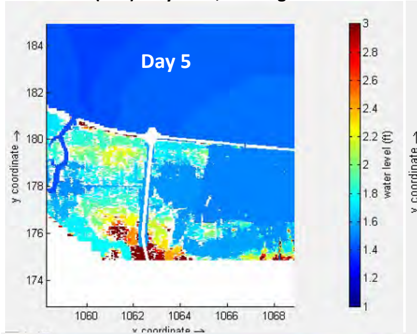
(20b) 25-yr rain, existing
