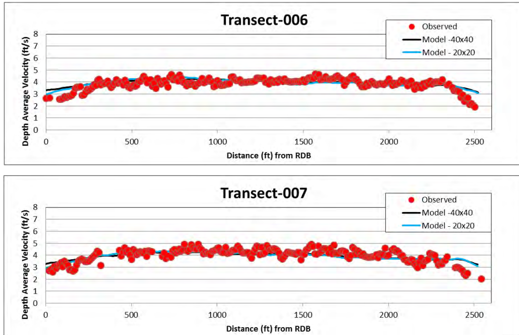
Figure A-4. Comparison between CFD model and field data at transects #006 and #007. Red dots show the field data and model results are given for two different meshes – 40x40 feet in size and 20x20 feet in size. The results with either mesh are similar.
