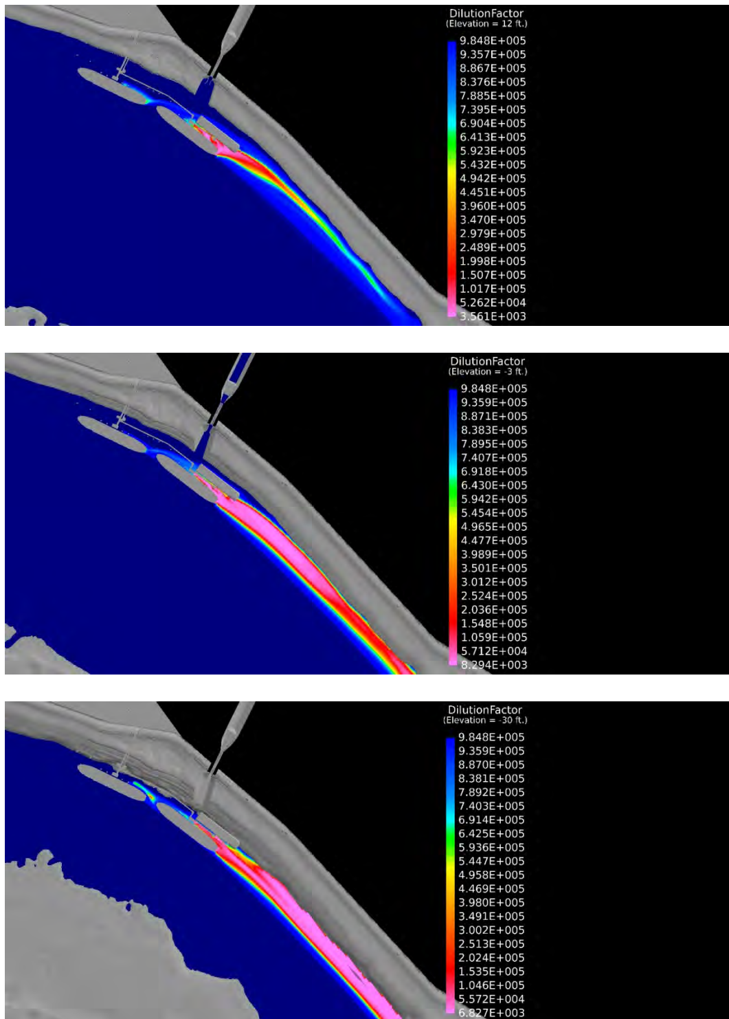
Figure A-17. Run #9 model results. Dilution factors at elevations 12 feet (top), -3 feet (middle), and -30 feet (bottom) 30 minutes after Bitumen spill.
