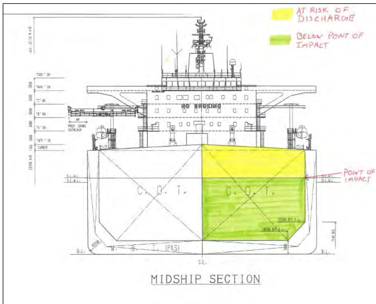
Figure A-26. Point of impact on the vessel (Run #10).
