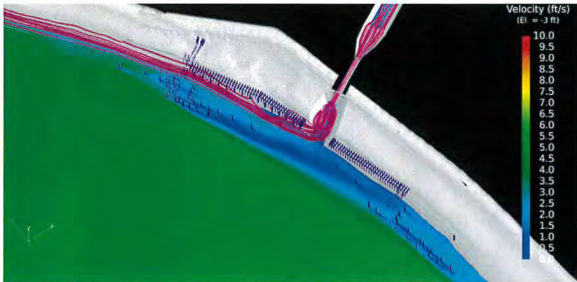
Figure 7 – Velocity contours with streamlines superimposed with Alternative 1 docking facility and operating diversion.
