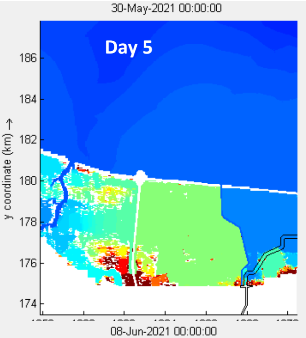
(21a) 2-yr rain, with-project, no div. flow
