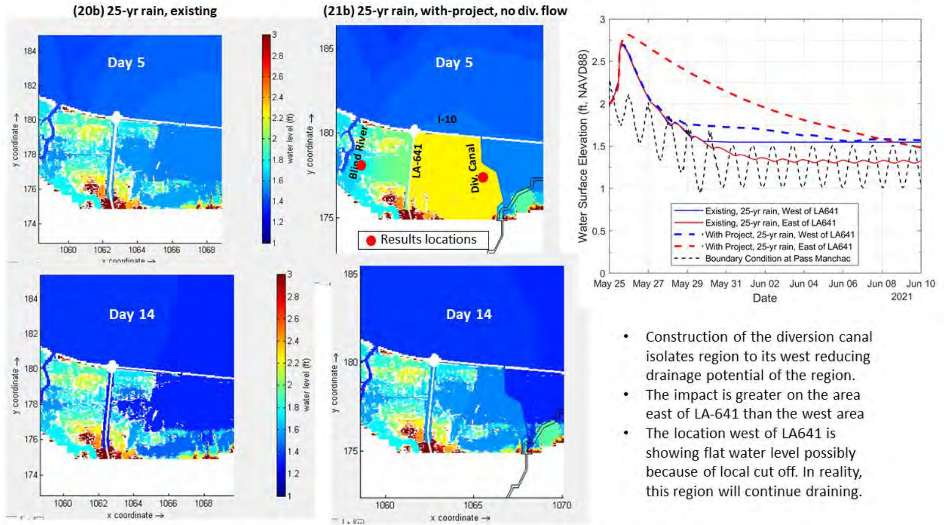
Figure G4. Comparison of existing and with-project, no diversion flow conditions (25-year rainfall).
