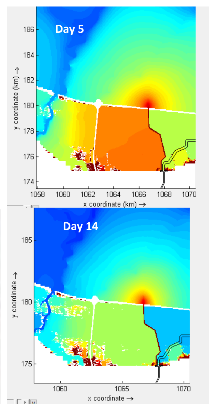
25-yr rain, with-project, div flow 2000 cfs
