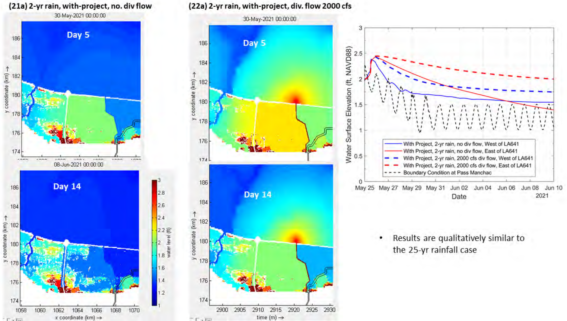
Figure G7. Comparison of with-project, no diversion flow and with-project, 2,000 cfs diversion flow conditions (2-year rainfall).
