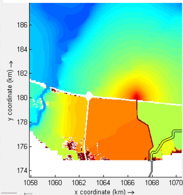
(22b) 25-yr rain, with-project, div flow 2000 cfs
