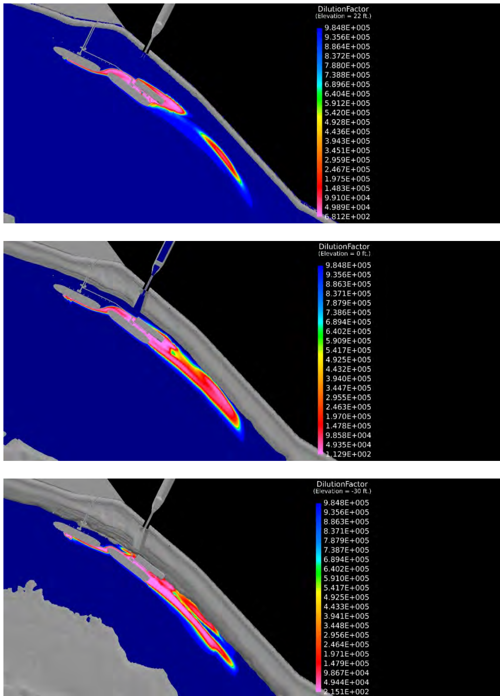
Figure A-20. Run #10 model results. Dilution factors at elevations 22 feet (top), 0 feet (middle), and -30 feet (bottom) 0.12 hour after Bitumen spill.
